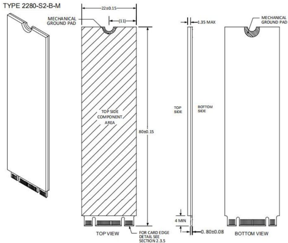
Figure 1 Dimension reference diagram (unit: mm)
