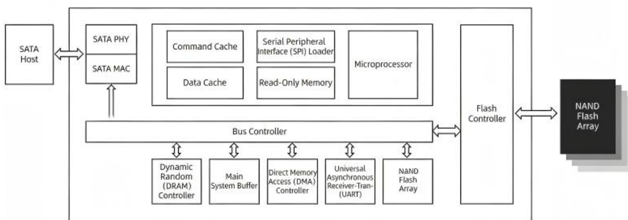
Figure 3 Block diagram of SSD control board product principle
